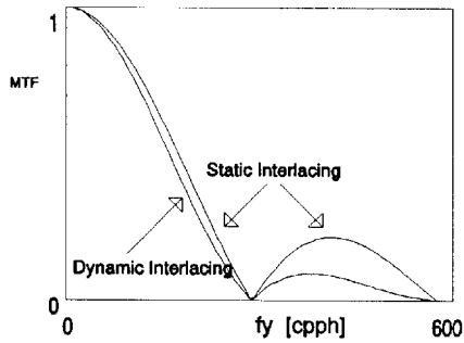
Figure 12: The MTF ( n=0 ) as a function of spatial frequency f_y in cycles per picture height [c/pps] for the ideal Static Interlaced case and the Dynamic Interlaced one. The first zero occurs at f_y=288 c/pps.
